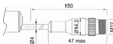
Pig-tail version
